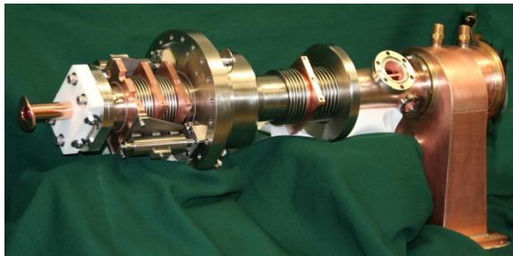
Figure 1: VWP3032 power coupler for Cornell.
